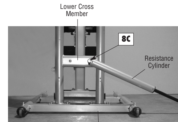
Base Frame Assembly
